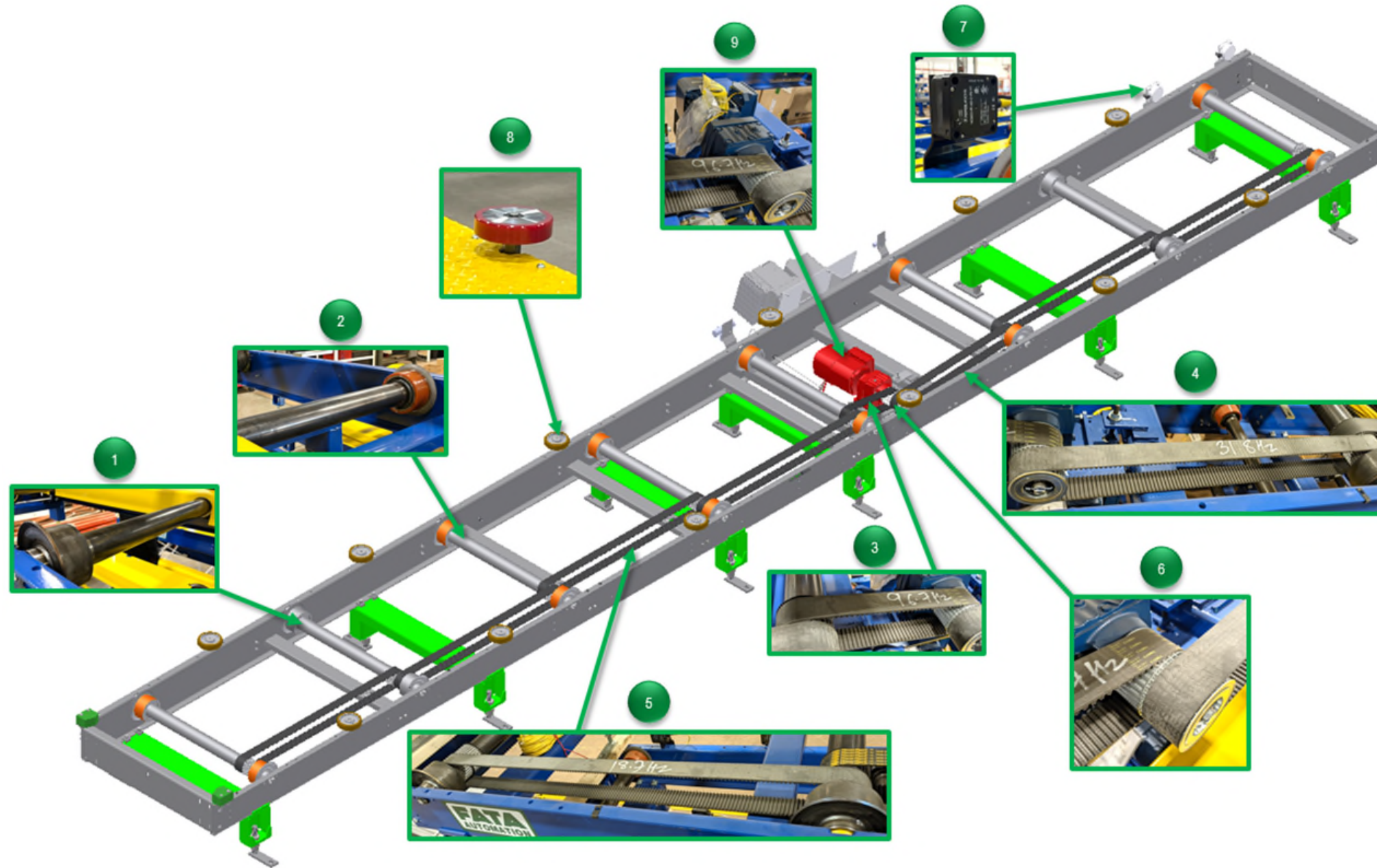
▲ Power Roll Bed - 3D rendition of 8 Roll shown with covers removed to show detail.
