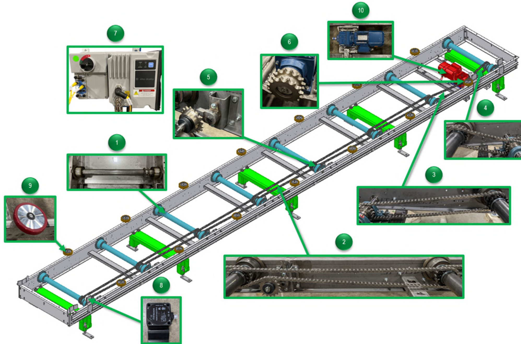
▲ Power Roll Bed - 3D rendition of 7 Roll shown with covers removed to show detail.
